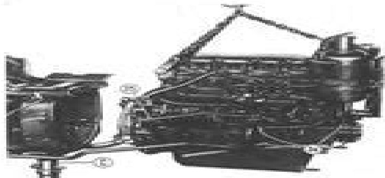
Fig. 8. - Removing the engine with lifting sling ARR 11366 and hoist.
