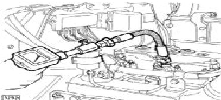
Checking engine compression using tester 291309.
