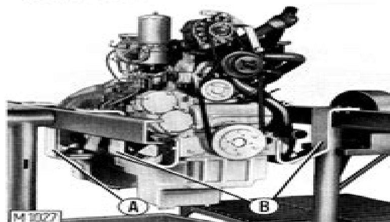
Fig. 2-5 Engine in position on Rotary stand 290090 A. - Rear brackets 293206 - B. Front brackets 293205.
