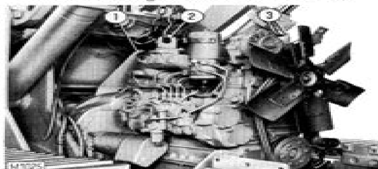
Fig. 2-3 Removal (Installation) of engine using lift hook 290740.
