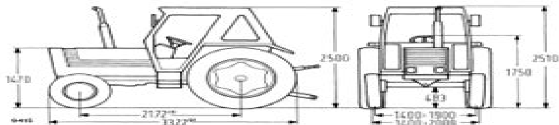
Mod. 680 (7.50-18 front and 13.6/12-38 rear tyres)
