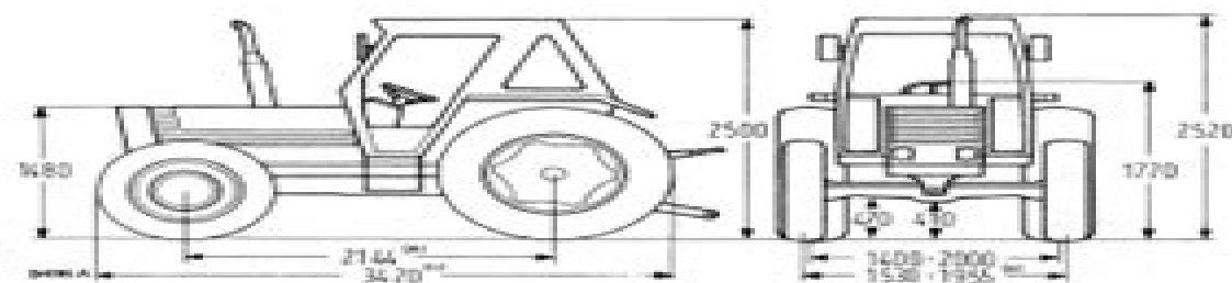
Mod. 680 DT (11.2/10-28 front and 13.6/12-38 rear tyres)
