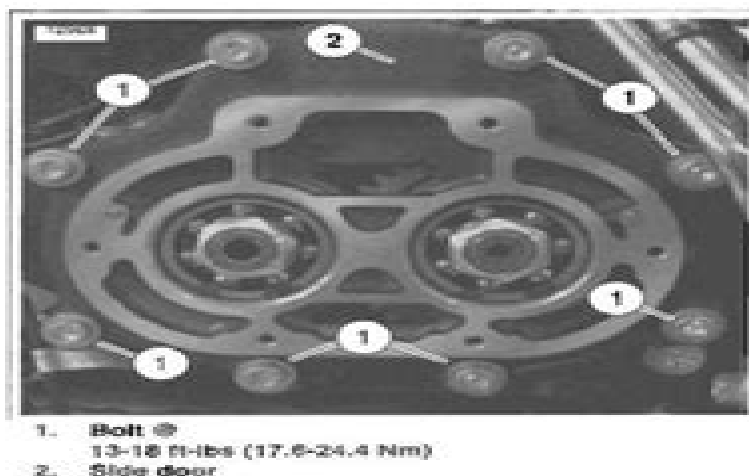
Figure 7-13. Side Door Hardware
