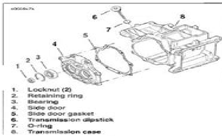
Figure 7-12. Side Door Bearings
