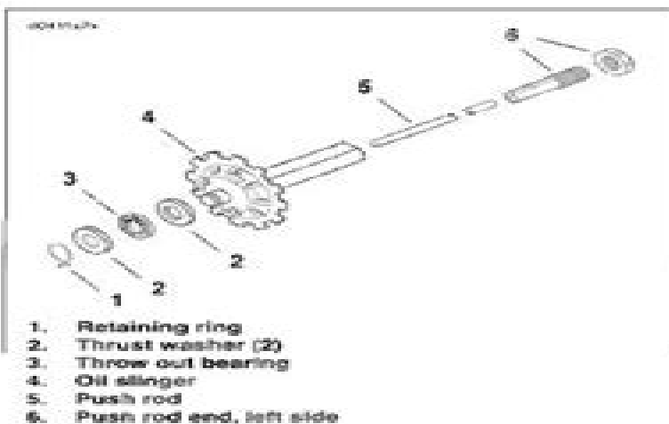
Figure 7-11. Push Rod Assembly
