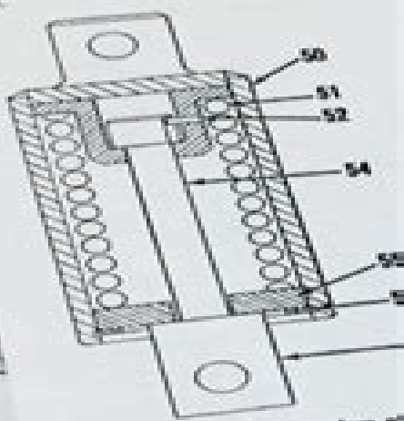
Fig. IH458C—Sectional view of roller plug assembly. Refer to text before disassembly.
