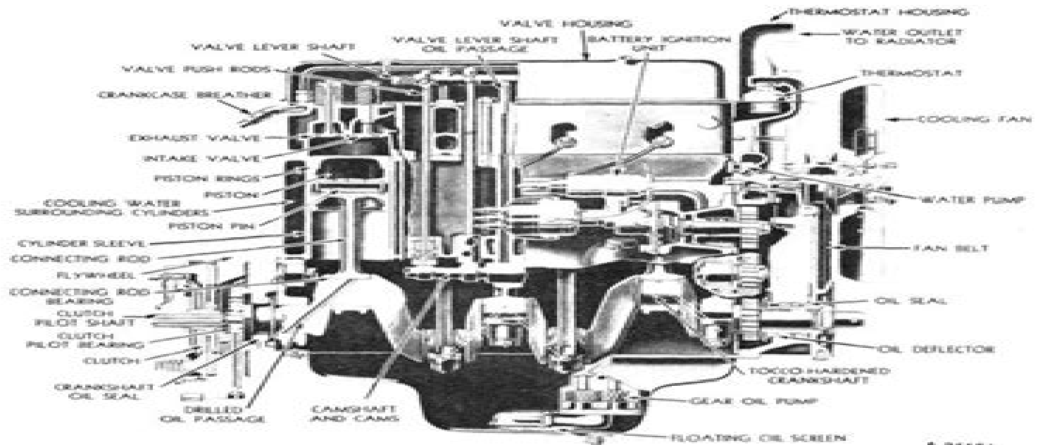
Cutaway view of Farmall H.
