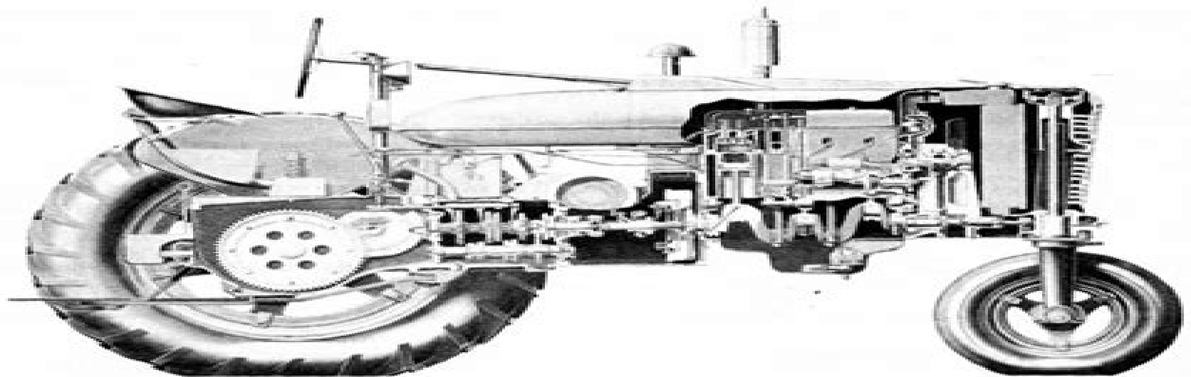
Cutaway view of Farmall H.
