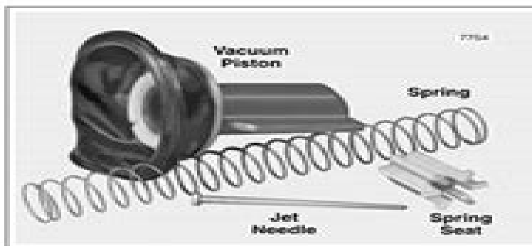
Figure 4-7. Carburetor-Top End
