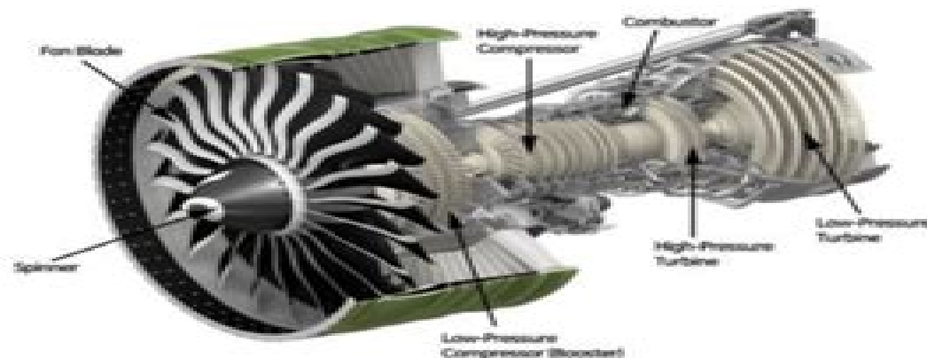
Fig. GE90-115B Turbofan cross-section
